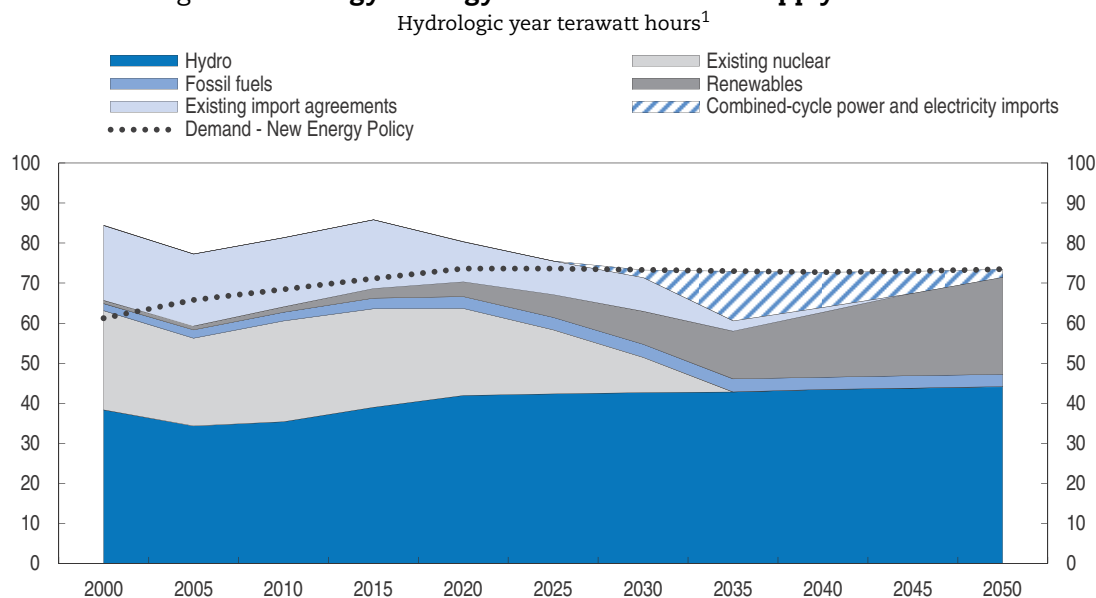
Figure 13. Energy Strategy 2050 demand and supply scenario
